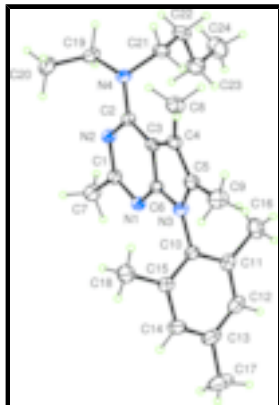
Fig. 1. Ellipsoids at the 50% level, with H atoms having arbitrary radius.
